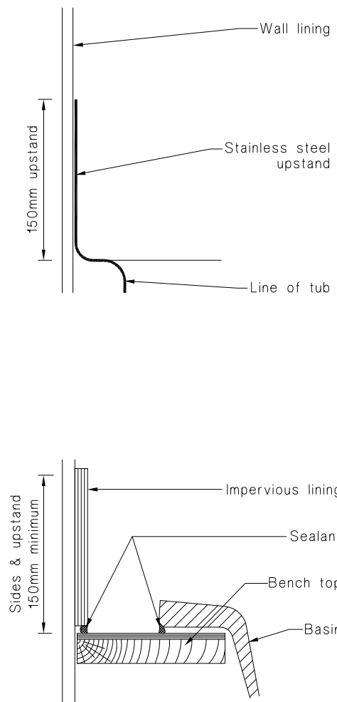
(b) Tub, sink and basin
