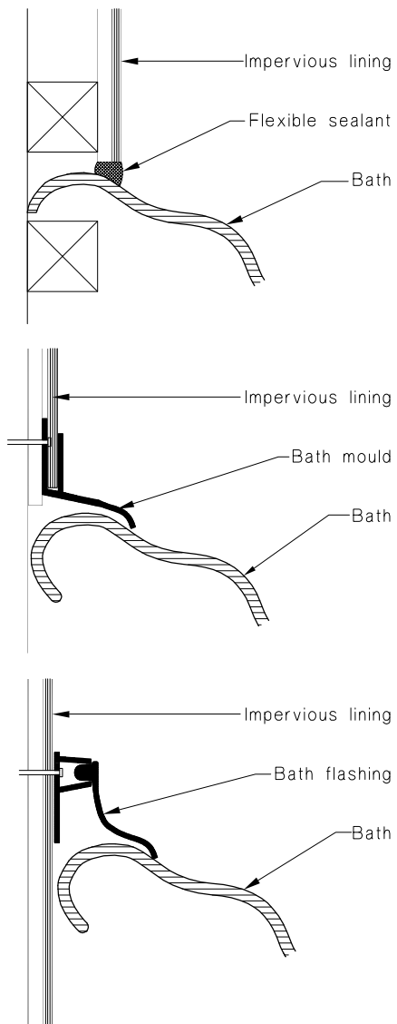
(a) Junctions of bath and wall
